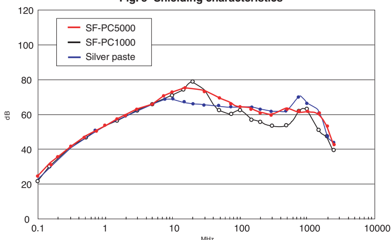
Fig. 5 Shielding characteristics
