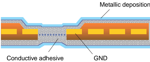
Fig. 3 Shielded FPC (Double-sided shielding)
