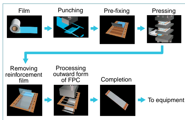
Fig. 9 Example of processing process for SF-PC1000
