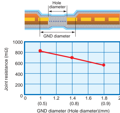
Fig. 8 Ground joint resistance (Double-sided shielding)
