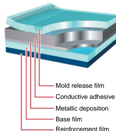
Fig. 1 Cross-sectional structure of the SF-PC1000
